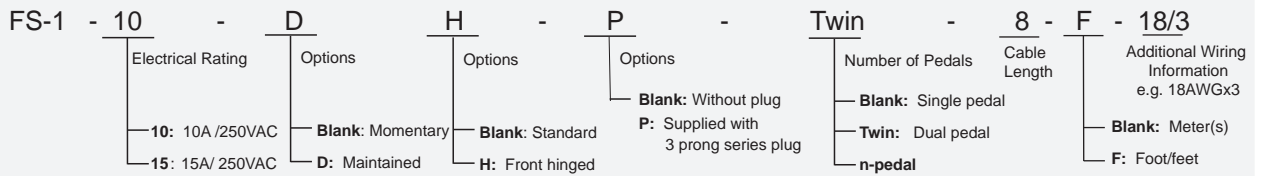
Standard model
