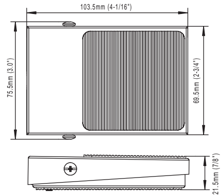
Standard model
